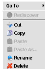
Figure 25 Right-click menu
